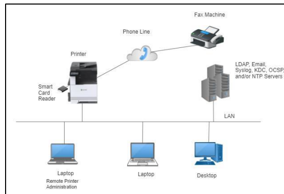
Figure 1: TOE Architecture
